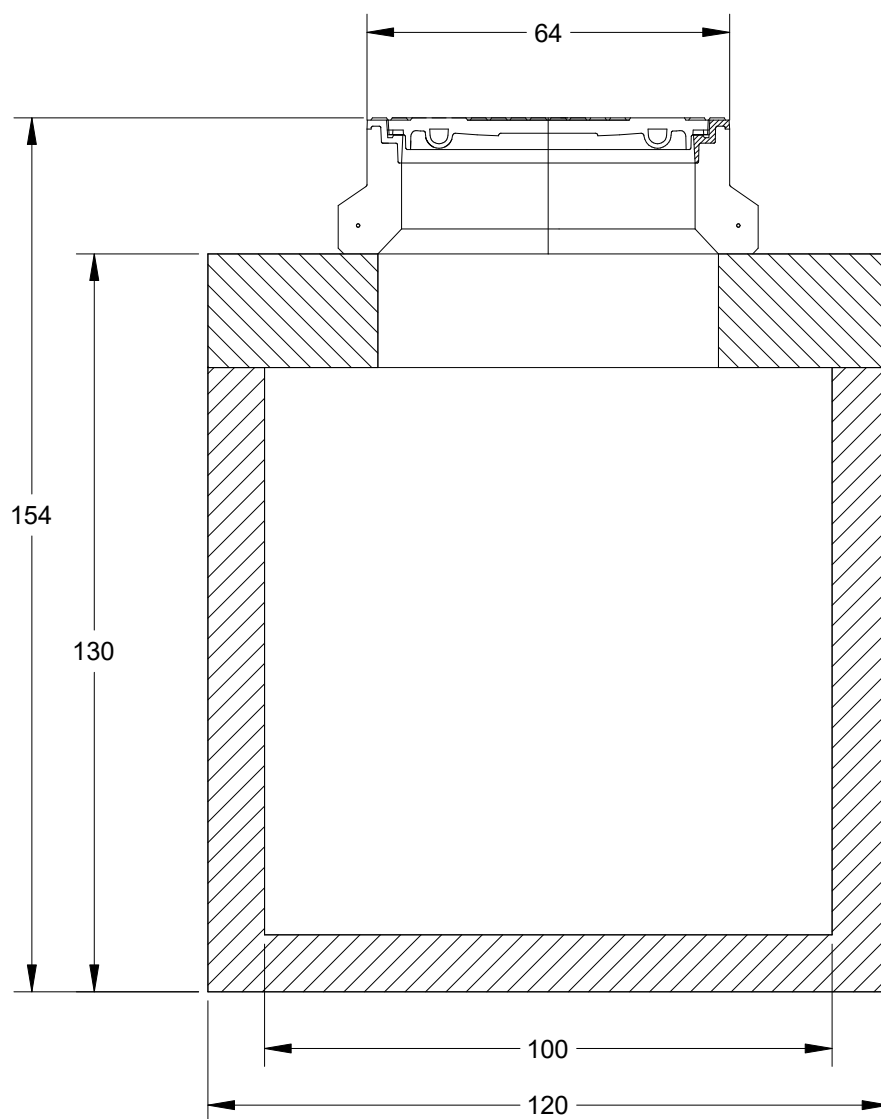
Betonput 120x120cm
