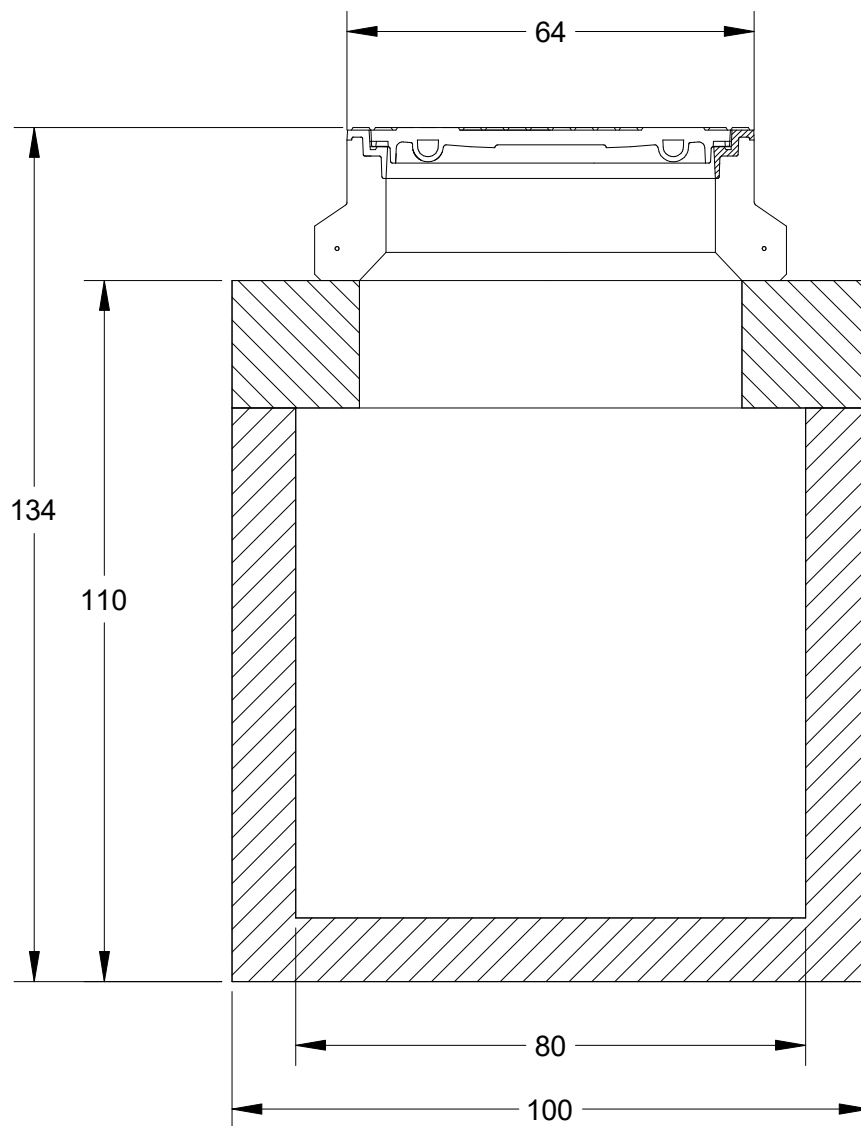
Betonput 100x100cm
